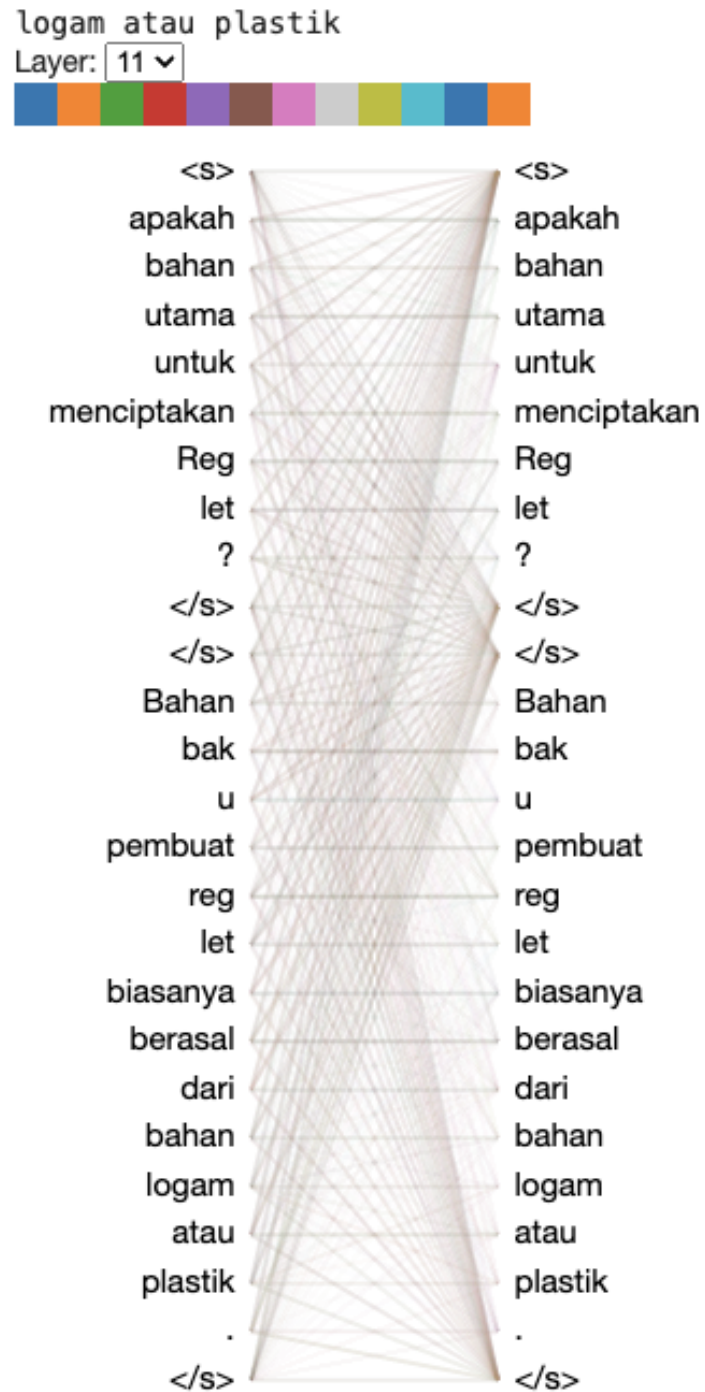
Figure 11: Binary classification attention: Indonesian, Layer 11. Answer displayed at top left.
